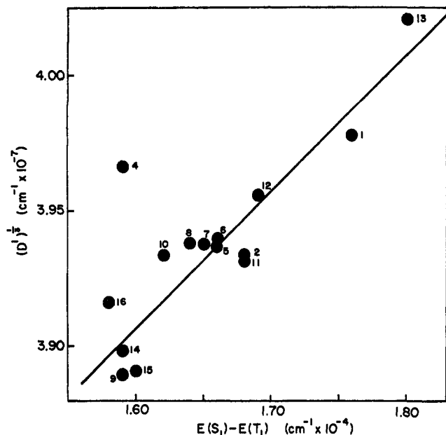
Figure 3. (D')^{1/3} vs. [E(S_1) - E(T_1)] . (D')^{1/3} = (hcD/g^2\beta^2)^{1/3} ( \text{cm}^{-1} ). The numbering of the points corresponds to that of the compounds listed in Table I.
