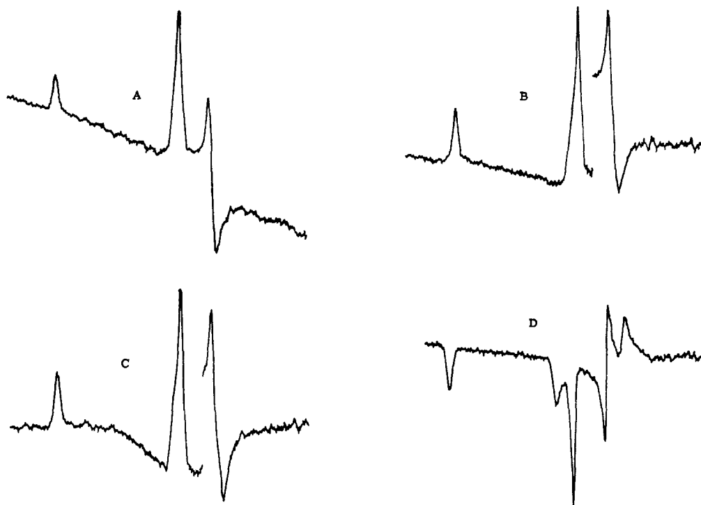
Figure 2. Epr spectra of the first excited triplet states of (A) 4,4'-diethylbiphenyl, (B) 4,4'-diisopropylbiphenyl, (C) 4,4'-di-sec-butylbiphenyl, and (D) 4,4'-di- tert -butylbiphenyl. Only the low-field half of the \Delta M = \pm 1 peaks is shown.
